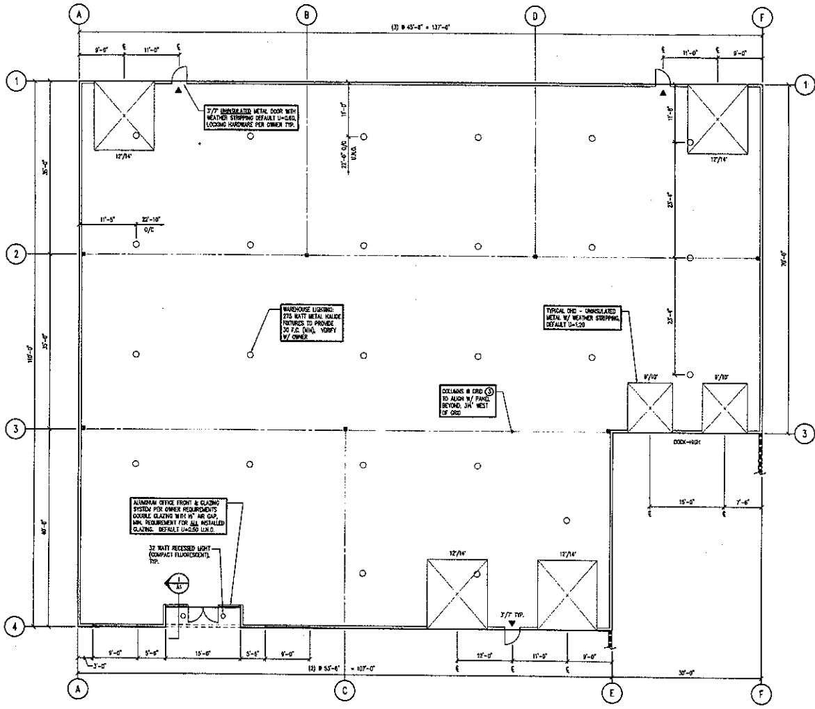
FLOOR PLAN - BUILDING "F" W'-1'-0" (13,870 S.F., 16' MIN. CLEAR)
