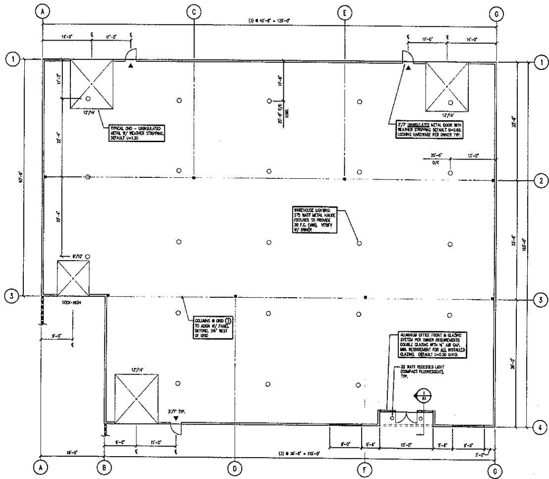
FLOOR PLAN - BUILDING "E" 1/8"=1'-0" (12,742 S.F., 16' MIN. CLEAR)
