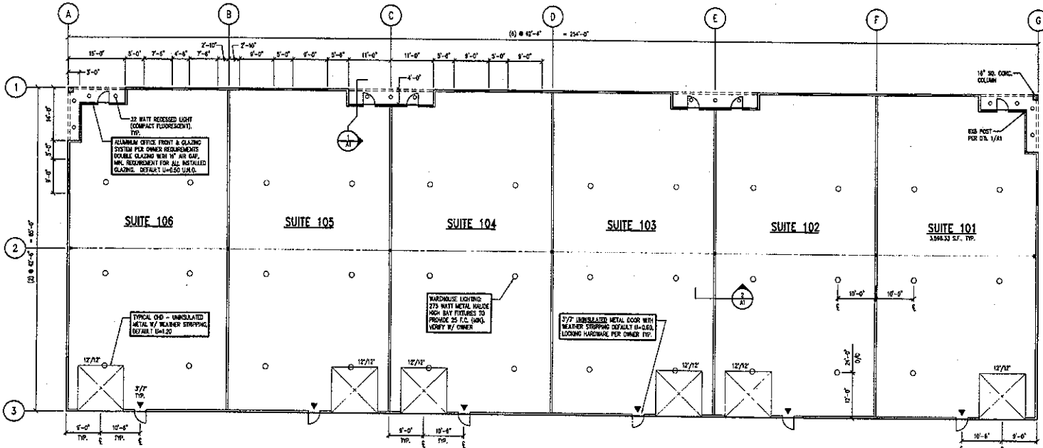
FLOOR PLAN - BUILDING "A" 1/8" = 1'-0" (21,590 S.F., 14' MIN. CLEAR)
